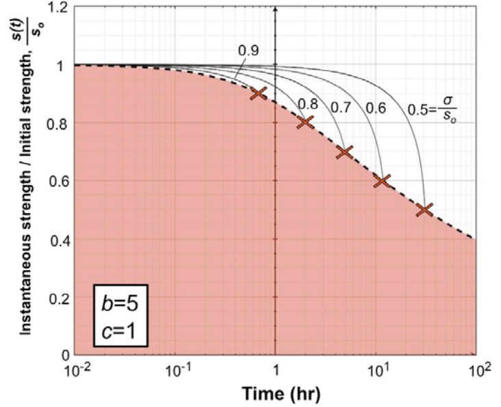
Figure 6. Strength decay with time.
