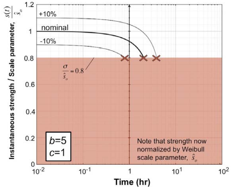
Figure 7. Time to failure accounting for variation in initial strength.
