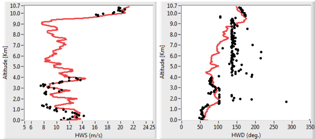
Fig. 6. Examples of dropsonde and DAWN AIR wind product comparisons. Horizontal Wind Speed (HWS) and Horizontal Wind Direction (HWD). FFT size = 2048. Exact noise floor for noise whitening. Line = Dropsonde, Dots = DAWN AIR.
