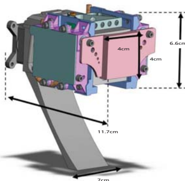
The STAMP Tool contains a tamper to smooth uneven surfaces, and a blade to excavate fresher subsurface material.
