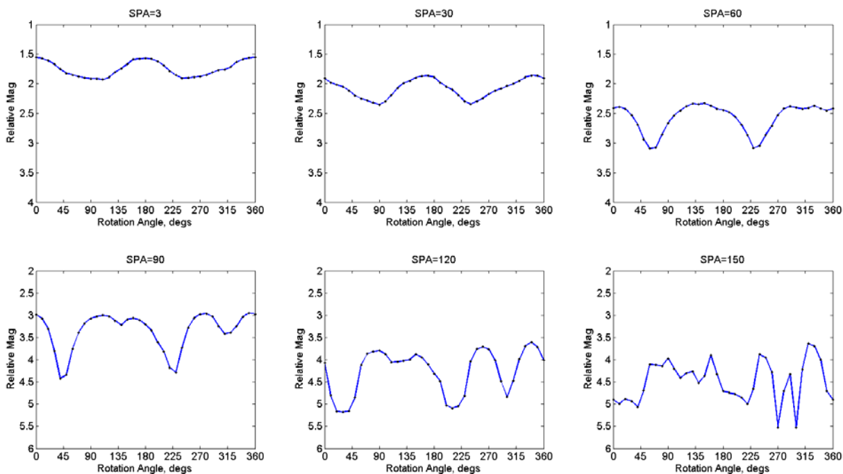
Figure 14. Relative magnitude lightcurves for white and orange rocket body in a spin-stabilized rotation using a clear filter.
