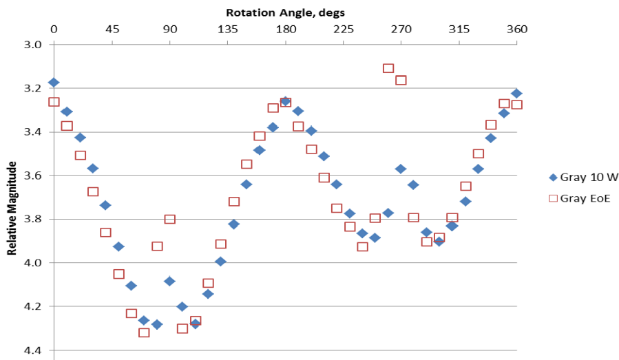
Figure 10. Relative magnitude comparison at 3^\circ SPA using gray rocket body for 10^\circ wobble (Gray 10 W) and end-over-end rotation (Gray EoE).
