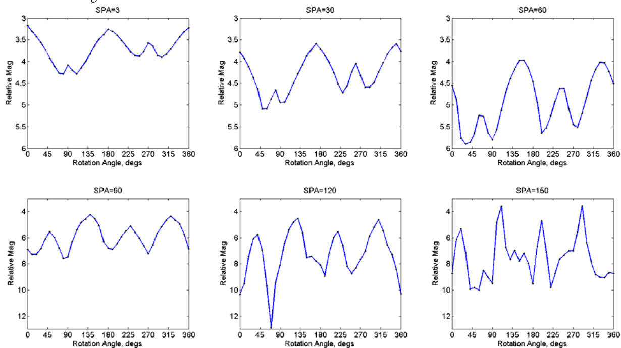
Figure 9. Relative magnitude lightcurves for gray rocket body rotated with 10^\circ wobble using a clear filter. Starting from top-left: SPA= 3^\circ , 30^\circ , 60^\circ , 90^\circ , 120^\circ and 150^\circ .
