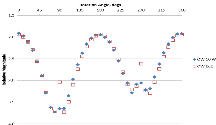
Figure 12. Relative magnitude comparison at 3° SPA using orange and white rocket body for 10° wobble (OW 10 W) and end-over-end rotation (OW EoE).
