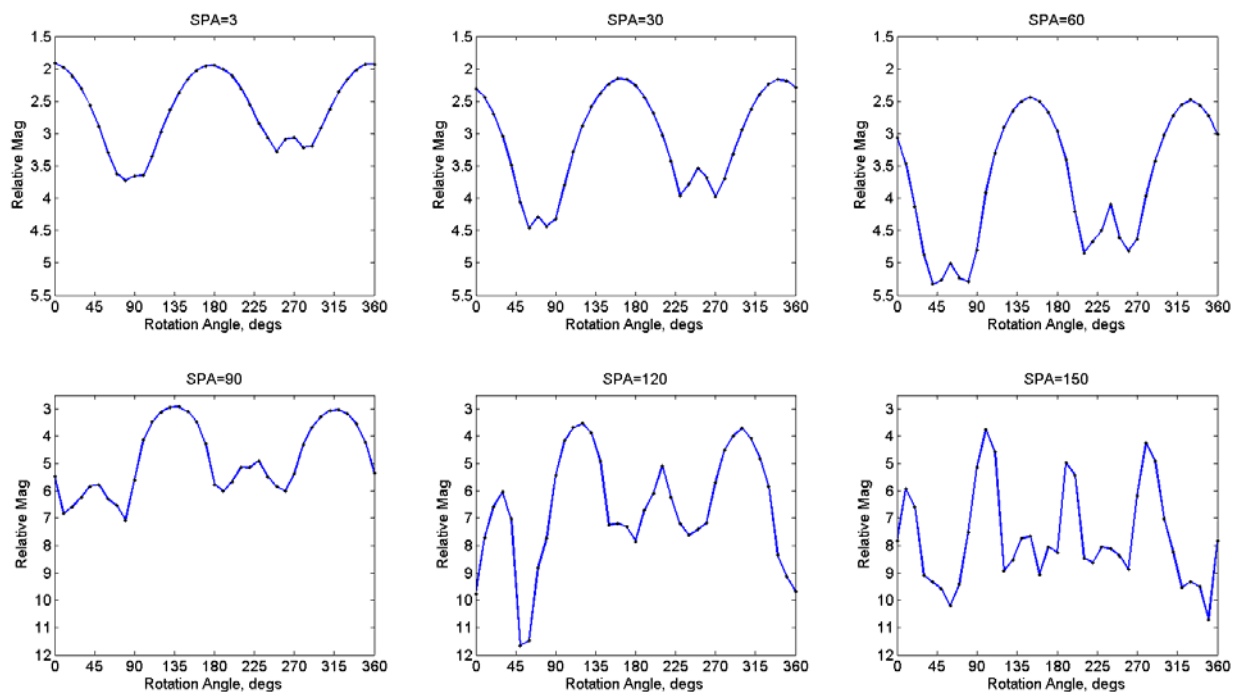
Figure 11. Relative magnitude lightcurves for white and orange rocket body rotated with 10° wobble using a clear filter. Starting from top-left: SPA=3°, 30°, 60°, 90°, 120° and 150°.
