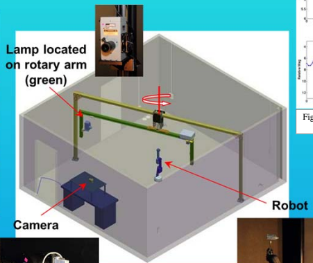
Figure 1. OMC layout for light source mounted on rotary arm, CCD camera, and robotic arm.
