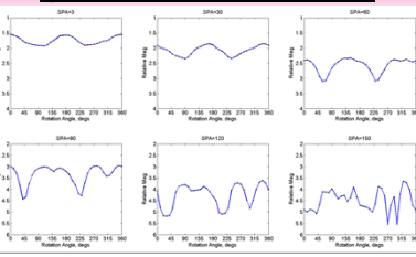
Figure 12. Relative magnitude lightcurves for white and orange rocket body in a spin-stabilized rotation using a clear filter.
