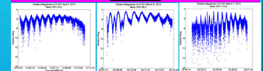
Figure 13: Telescopic data for SSN 21231 (has not been normalized or range corrected): (Left) April 3rd, 2012. <SPA>=33.6°, SPA range 65.9°-12.0°. (Middle) March 6th, 2012. <SPA>=96.5°, SPA range 93.6°-98.6°. (Right) March 7th, 2012. <SPA>=114.8°, SPA range =107.8°-118.5°.
