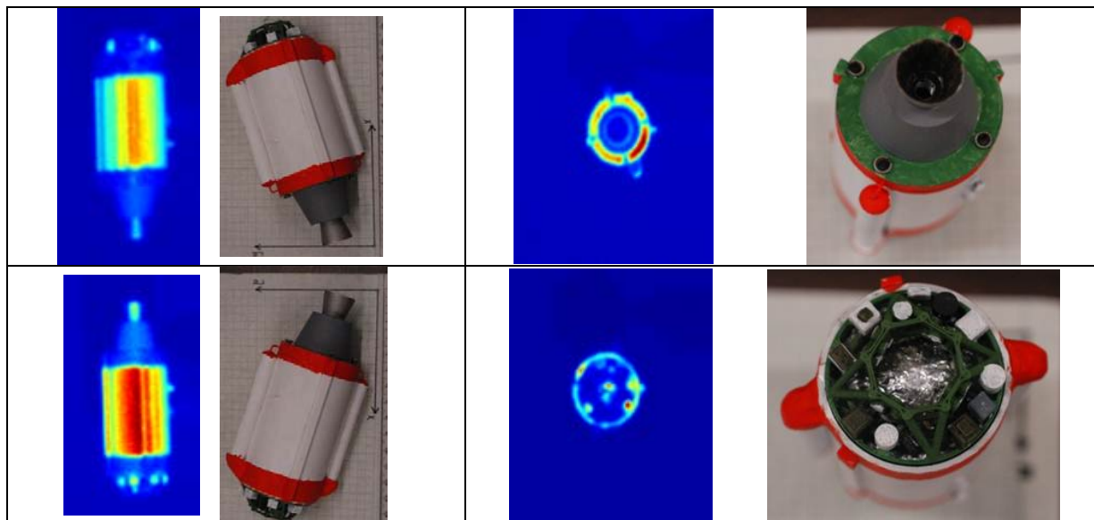
Figure 3. Left quad-plot: Raw imagery data taken with SBIG CCD using a clear filter showing the OMC rotation sequence for end-over-end orientation (no background subtraction has been applied). Photographs are aligned with rotations representing the side view, thrust end, opposite side view and payload end.
