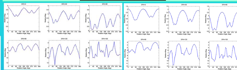
Figure 7. Relative magnitude lightcurves for gray rocket body rotated with 10° wobble.
