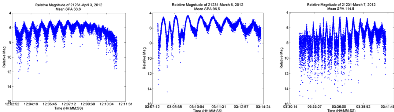
Figure 5. (Left) Lightcurve plot for SSN 21231 on April 3rd, 2012. \langle \text{SPA} \rangle = 33.6^\circ , SPA range 65.9^\circ - 12.0^\circ . (Middle) Lightcurve for SSN 21231 on March 6th, 2012. \langle \text{SPA} \rangle = 96.5^\circ , SPA range 93.6^\circ - 98.6^\circ . (Right) Lightcurve for SSN 21231 on March 7th, 2012. \langle \text{SPA} \rangle = 114.8^\circ , SPA range = 107.8^\circ - 118.5^\circ .
