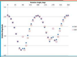
Figure 10: Relative magnitude comparison at 3° SPA using orange and white R/B for 10° wobble (OW 10W) and end-over-end rotation (OW EOE).
