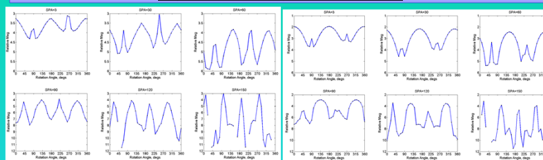
Figure 5. Relative magnitude lightcurves for gray rocket body rotated end-over-end.
