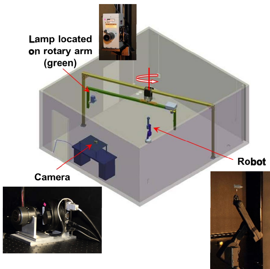
Figure 1. OMC layout for light source, CCD camera, and robotic arm.
