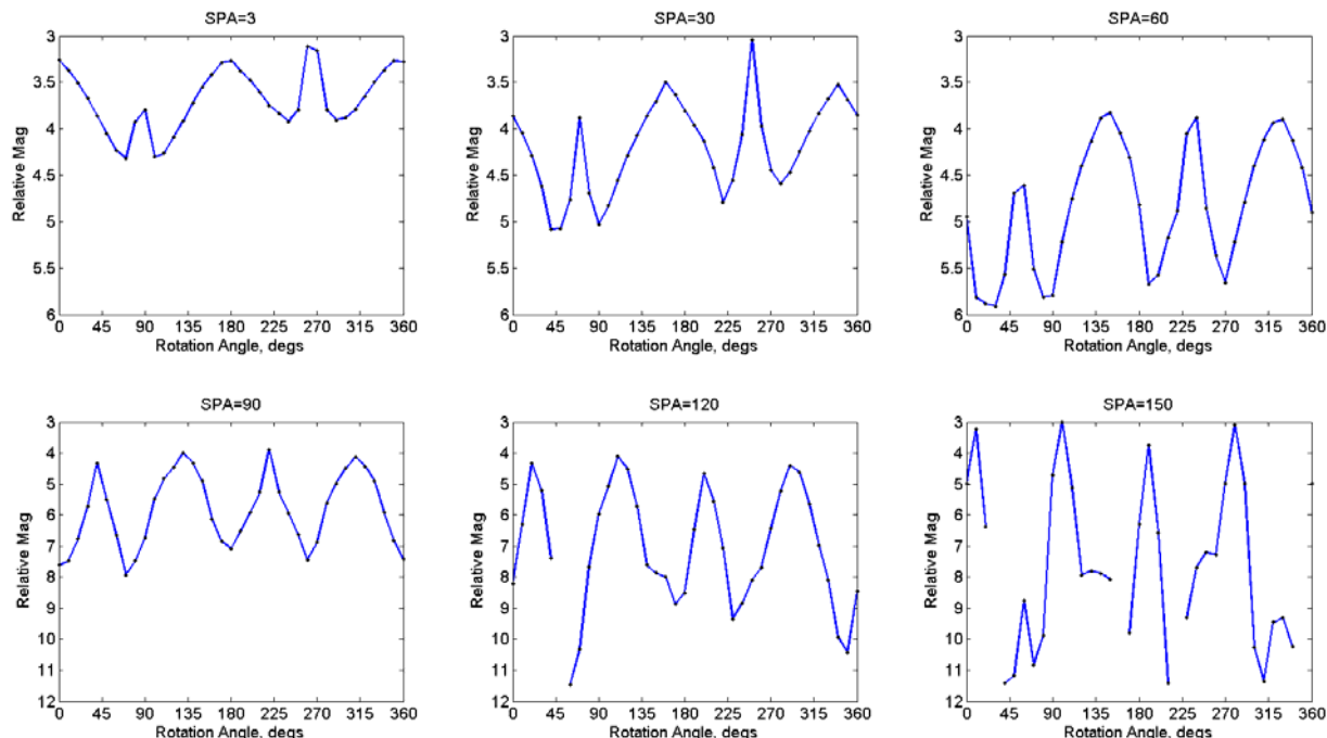
Figure 4. Relative magnitude lightcurves for gray rocket body rotated end-over-end using a clear filter. Starting from top-left: SPA=3°, 30°, 60°, 90°, 120° and 150°.
