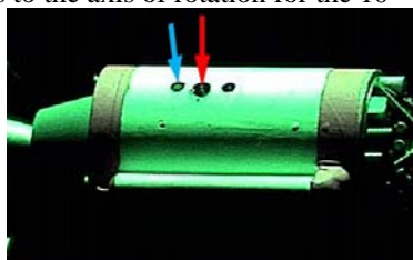
Figure 8. Mount holes on rocket body for robotic arm. Blue arrow points to 10 degree wobble mount and red arrow points to end-over-end rotation mount, which passes through the center of mass. The non-specified hole to the right of the red arrow is for future measurements.
