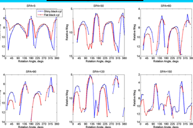
Figure 11. Relative magnitude for shiny black simple cylinder and flat, matte black cylinder in an end-over-end rotation.
