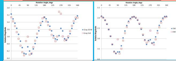
Figure 9: Relative magnitude comparison at 3° SPA using gray R/B for 10° wobble (Gray 10W) and end-over-end rotation (Gray EOE).
