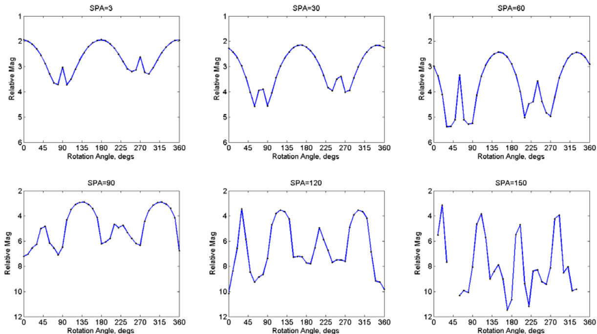
Figure 6. Relative magnitude lightcurves for white and orange rocket body rotated end-over-end using a clear filter. Starting from top-left: SPA=3°, 30°, 60°, 90°, 120° and 150°.
