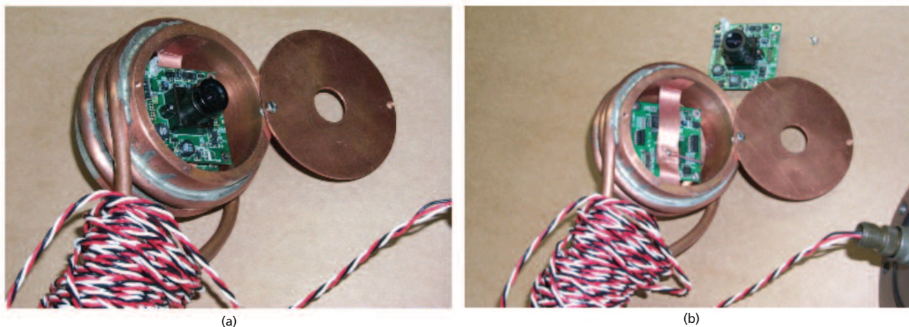
Photos of Vacuum Camera Cooler: (a) Camera cooler with camera installed and (b) camera cooler with camera partially removed to expose copper tape and thermocouple, which are attached to overheating camera CPU.
