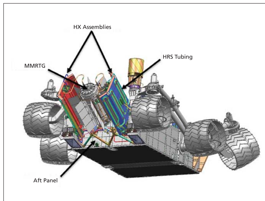
MSL Rover in Stowed Cruise Configuration showing HXs positioned on both sides of finned MMRTG.
