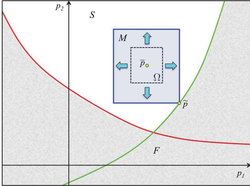
Figure 3. Maximal safe set of a hyper-rectangular reference set.
