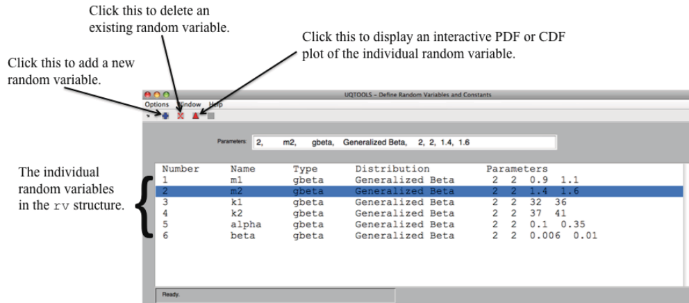
Figure 1. uqtools_gui main window.
