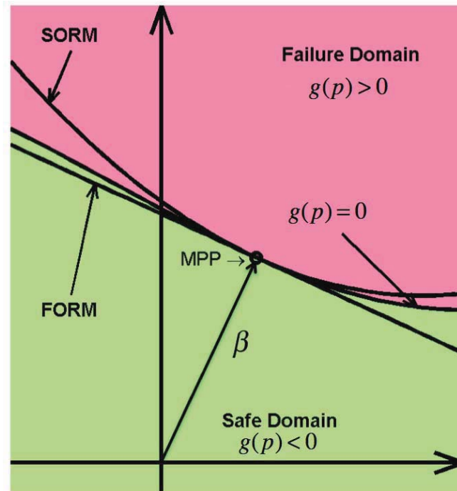
Figure 5. FORM and SORM
