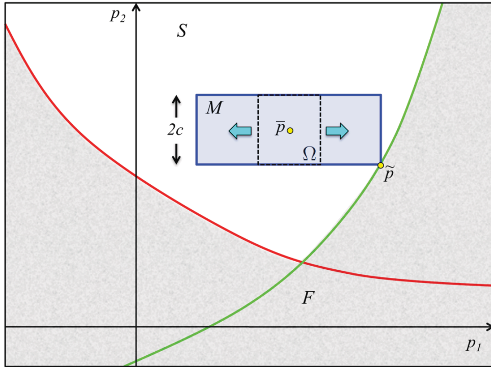
Figure 4. Hold some variables fixed, adjust others to find maximal safe set.
