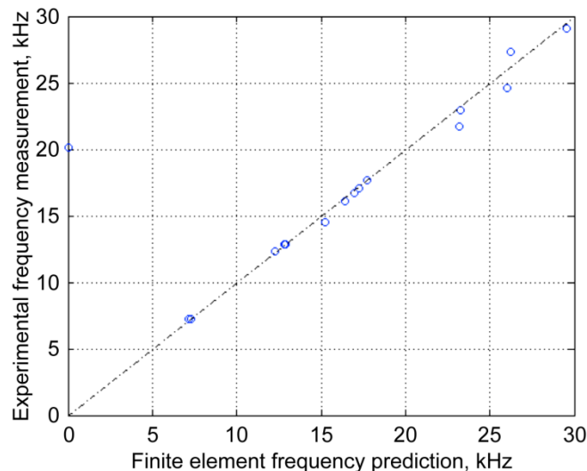
Figure 9.—Comparison of experimental and finite element natural frequencies.
