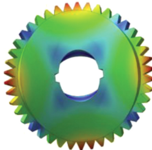
Mode 7, 7780 Hz
