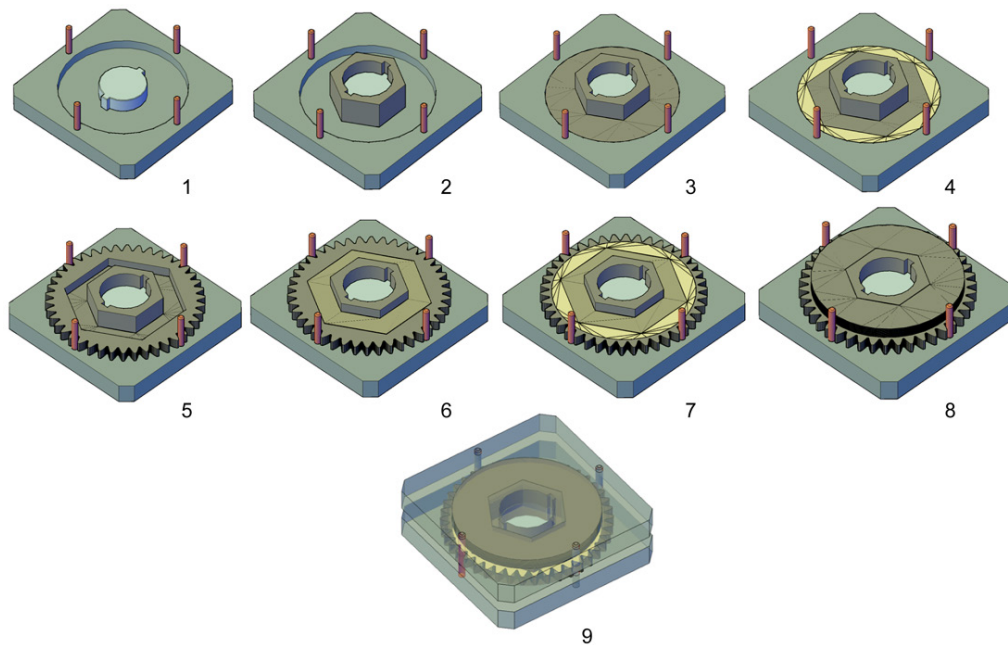
Figure 1.—Hybrid gear assembly steps.
