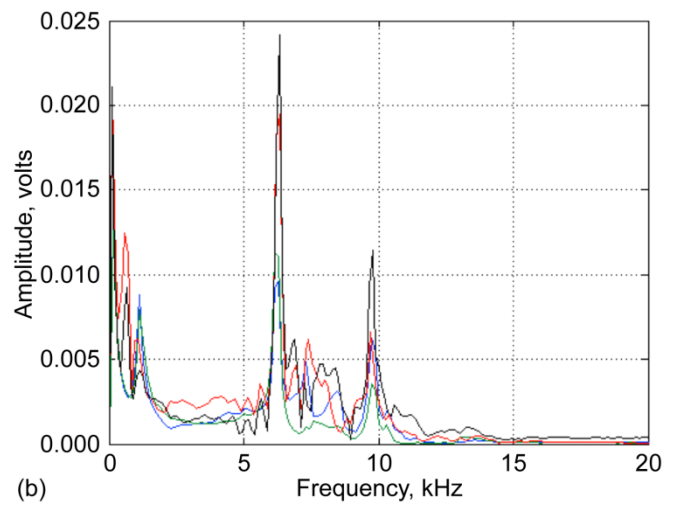
Figure 6.—Frequency domain results, axial location impacts. All steel gear. (b) Hybrid gear.
