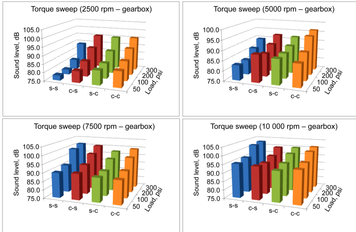
Figure 12.—Sound level measurements made for the four different test arrangements made at four different speed and load conditions.
