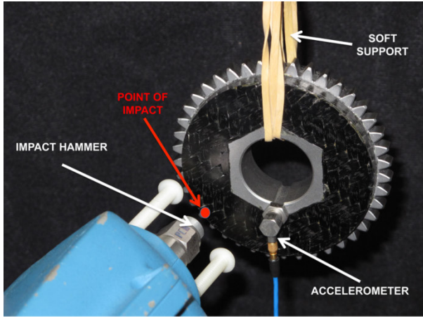
Hybrid gear, axial impact
