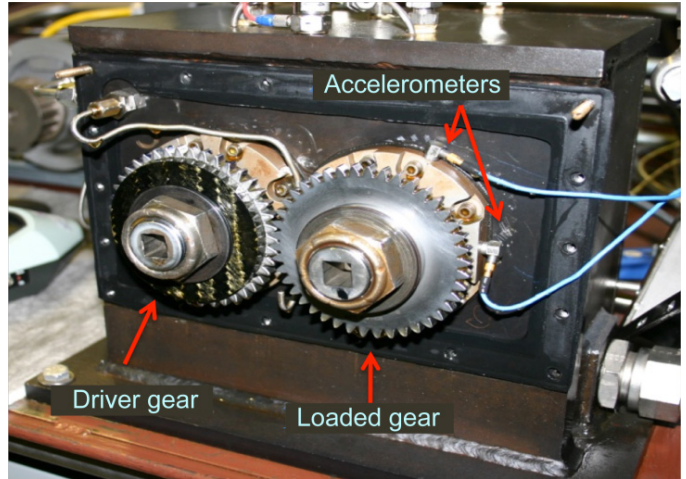
Figure 10.—Test facility shown with cover removed. Accelerometers are located on the right side driven gear. The hybrid—all steel gear arrangement shown in the photograph.
