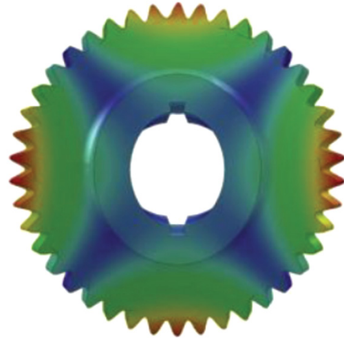
Mode 7, 7186 Hz
