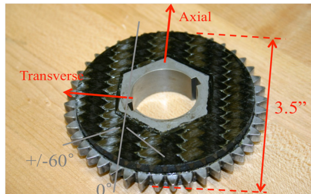
Figure 2.—Hybrid gear.
