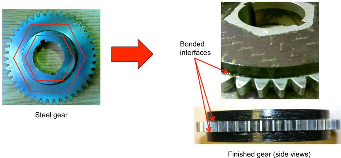
Figure 3.—Hybrid gear manufacturing details.
