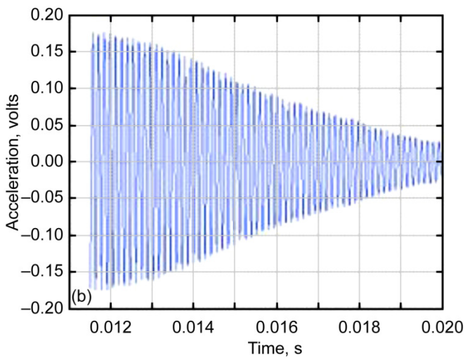
Figure 5.—Sample data raw. (a) Time domain signal. (b) Filtered data.
