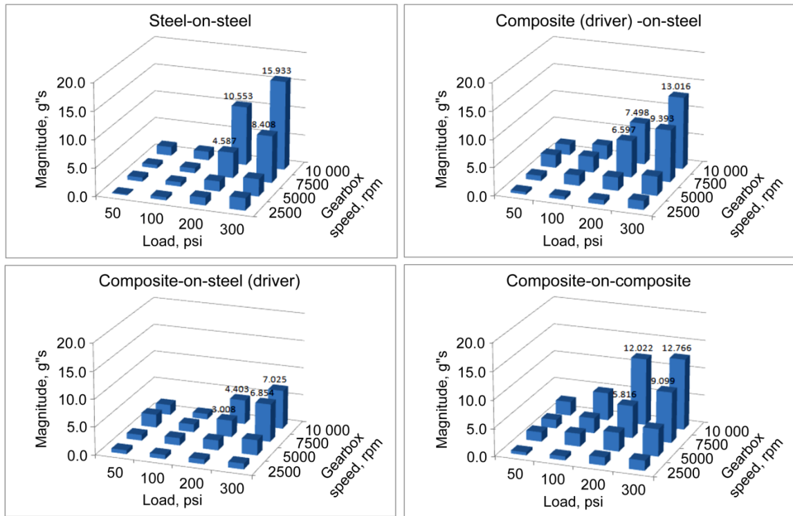
Figure 11.—Vibration data taken for four speeds and four load levels.
