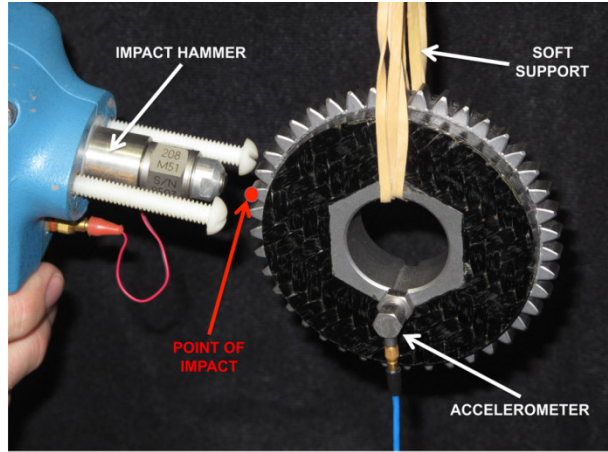
Hybrid gear, radial impact
