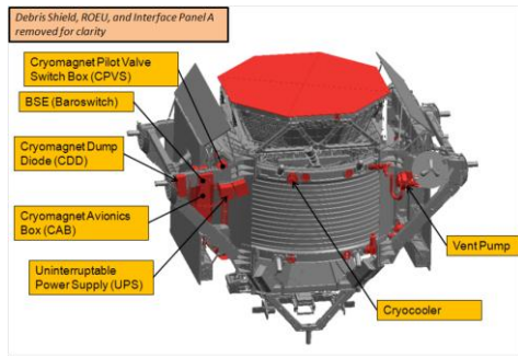
Figure 6. Schematic Diagram Illustrating Removed Electrical and Electronic Components
