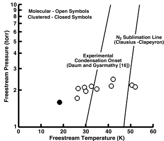
Fig. 5 Demonstration of significant freestream supercooling in N 2 beyond the condensation onset limit in the AEDC T9 wind tunnel (taken from [37]).
