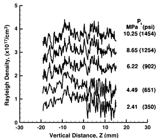
Fig. 2 Measured average freestream density.
