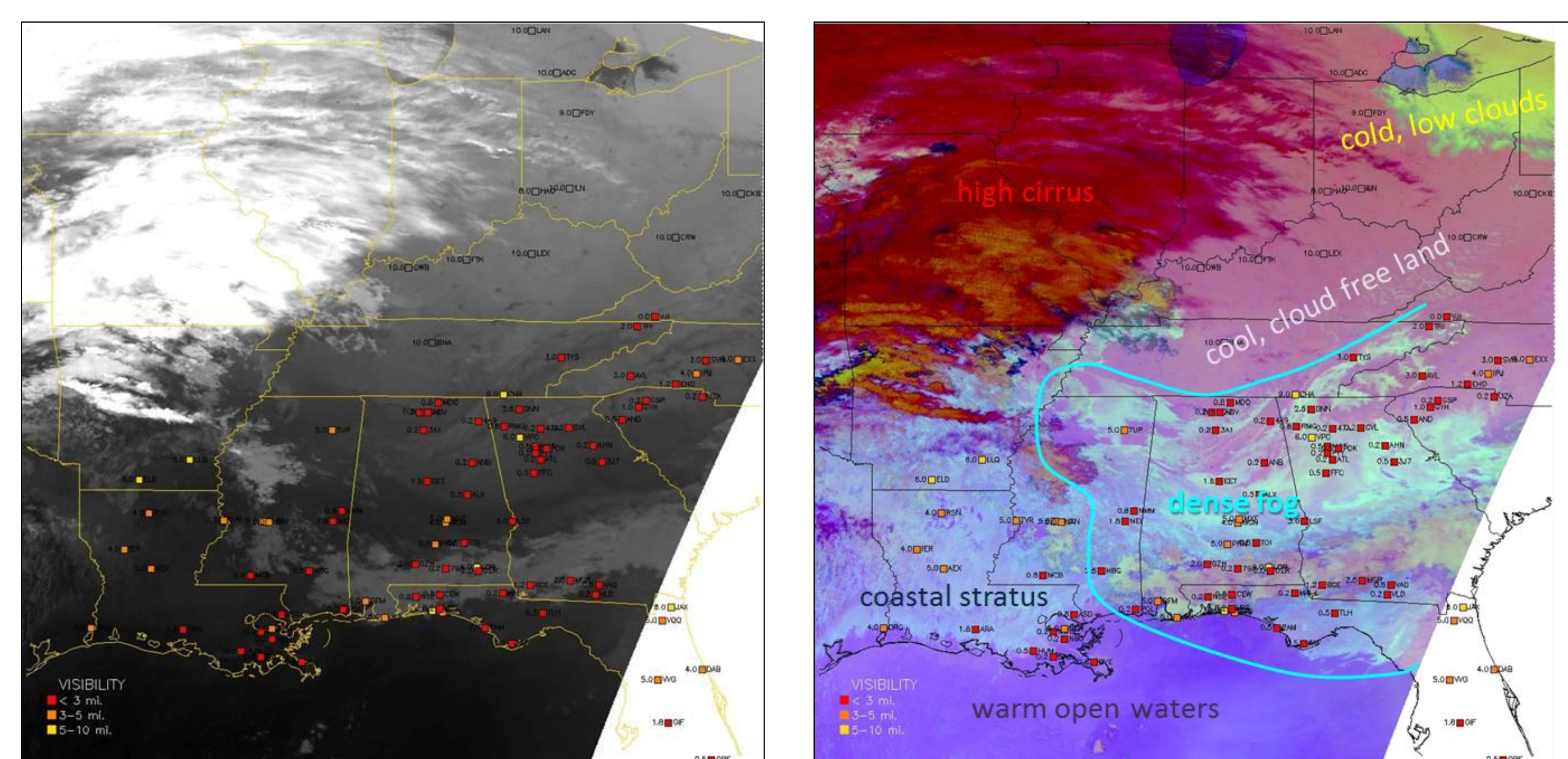
Figure 2. Comparison of single channel infrared data and multispectral RGB night microphysics imagery for a fog event at 0815 UTC on 24 November 2010. Data were acquired from the MODIS instrument aboard the Aqua satellite and processed according to EUMETSAT guidelines.
