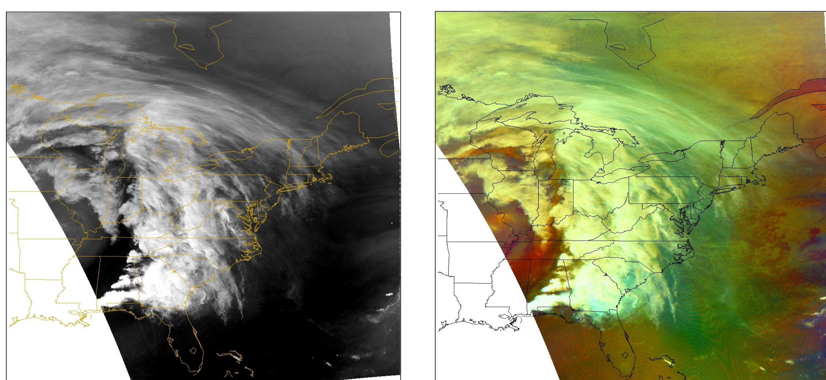
Figure 3. Comparison of single channel water vapor imagery and multispectral RGB air mass imagery for a severe weather event occurring across the southeastern United States at 0315 UTC on 16 April 2011. Data were acquired from the MODIS instrument aboard the Aqua satellite and processed according to EUMETSAT guidelines.
