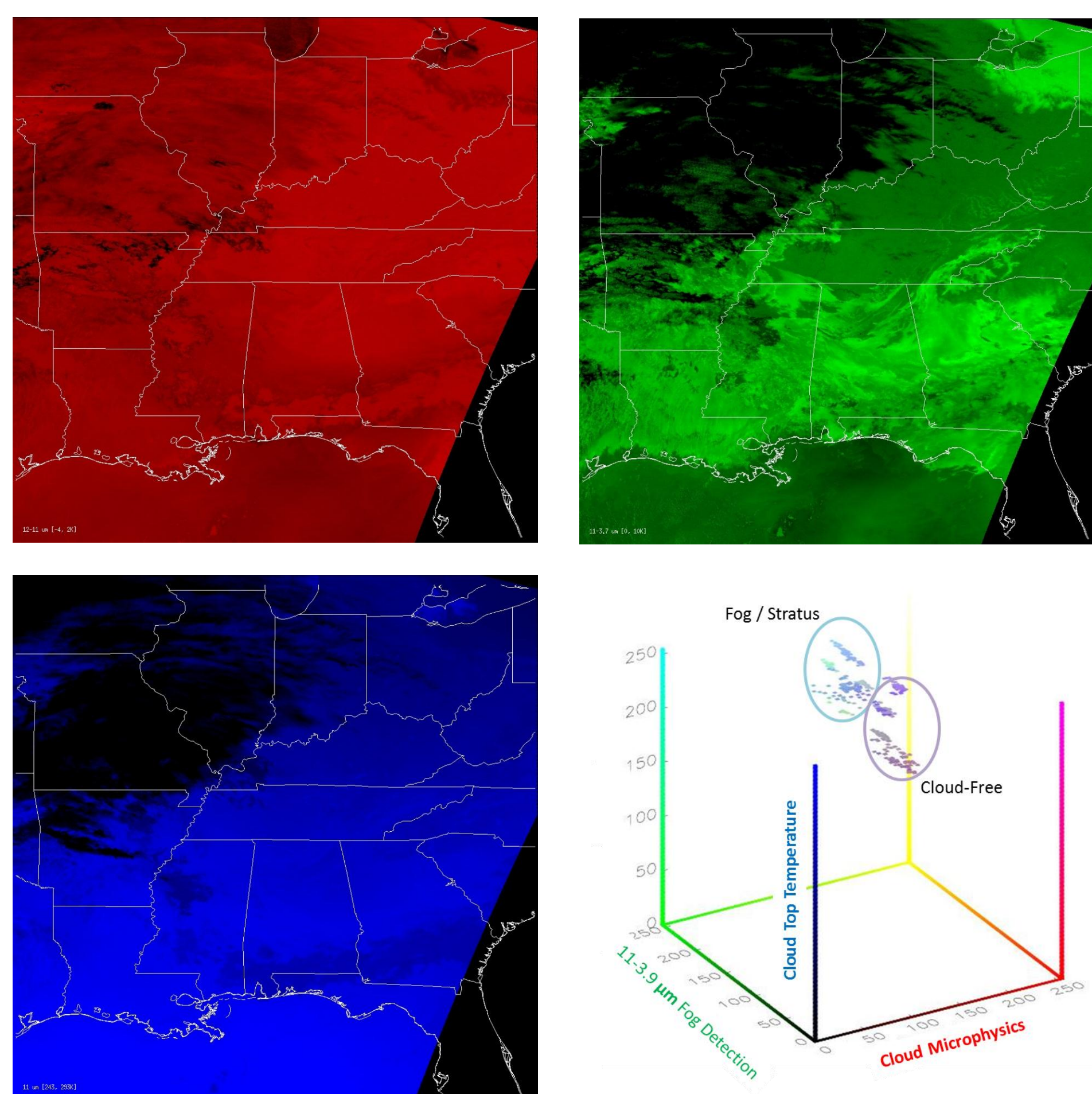
Figure 1. An example of the red, green, and blue color inputs to the “Nighttime Microphysics” product, based upon EUMETSAT guidelines, and separation of features by color.
