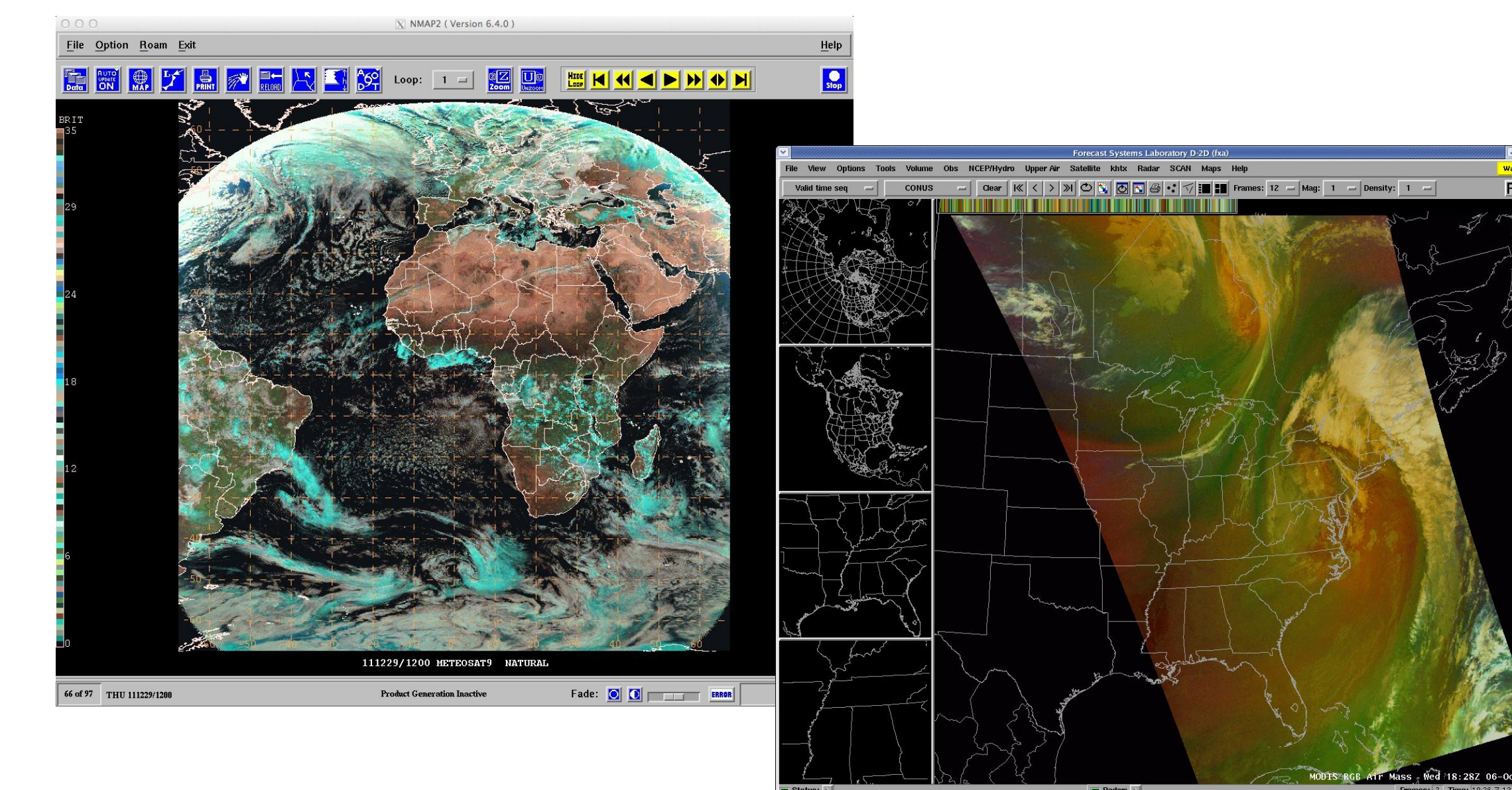
Figure 6. Examples of SEVIRI natural color product displayed in the current version of NAWIPS, and example of a MODIS air mass product displayed in AWIPS. These systems are used at NOAA/NWS Weather Forecast Offices and National Centers to integrate various data sets.
