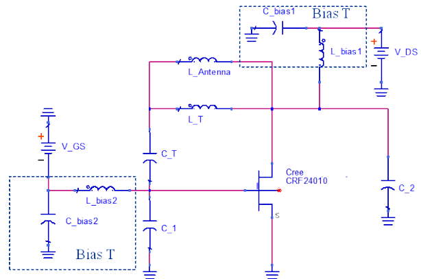
Figure 3: Schematic of wireless circuit for seismometer.
