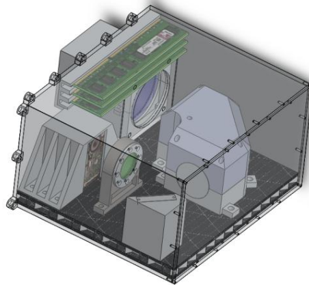
Fig. 32: Emulated spectrometer.
