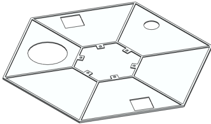
Fig. 4: Aluminum nadir hexagonal panel. The panel includes access and mounting holes for components, as well as webbing for increased structural rigidity.
