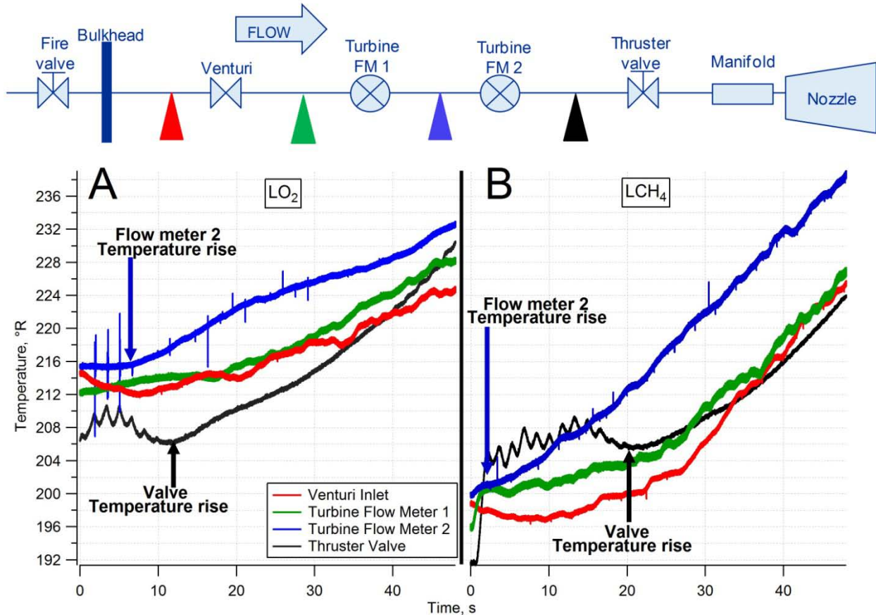
Figure 16.— Feed system temperatures for (A) LO 2 and (B) LCH 4 lines. Corresponding sensor locations are show in the above schematic.
