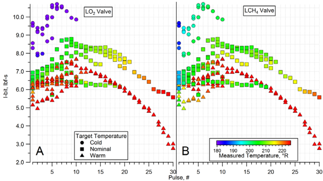
Figure 7.— I-bit for each pulse with propellant inlet temperature at the (A) LO 2 and (B) LCH 4 thruster valves. Only 80ms EPW runs with 1 st pulse temperatures within \pm 10^\circ\text{R} of the target are shown.
