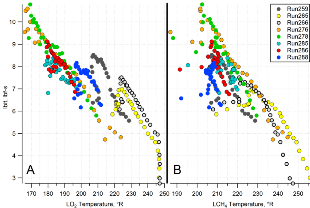
Figure 8.— I-bit as a function of (A) LO 2 and (B) LCH 4 inlet temperature for 30 pulse tests.
