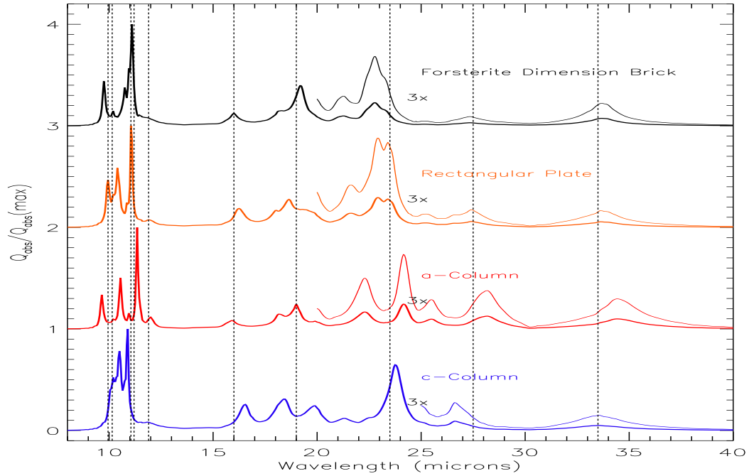
Figure 1: DDSCAT calculated Q_{qabs} for a_{eff} = 0.1 \mu\text{m} analogs to the bulky, platy, and columnar/needle forsterite condensates presented in [7]. From top-to-bottom, bulky = forsterite dimension brick ( black ), platy = rectangular plate ( orange ), and columnar/needle = a-Column ( red ) and c-Column ( blue ). The number of dipoles, i.e. lengths, along the optical a-, b-, and c- axes are 14 \times 7 \times 18 , 60 \times 15 \times 15 , and 15 \times 15 \times 60 for the rectangular plate, a-Column, and c-Column, respectively. The far-IR Q_{abs} values have been multiplied by 3 to increase feature contrast.
