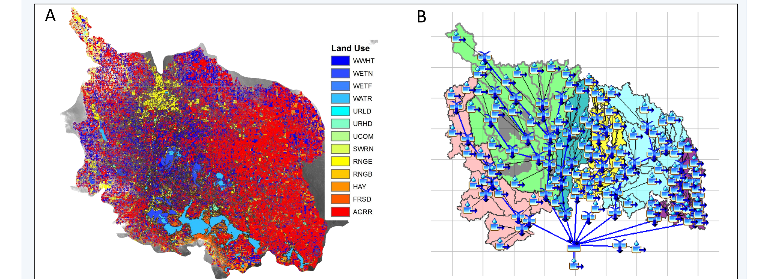
Figure 7. Land use (A) and HEC-HMS watershed delineation (B). Abbreviations: WWHT: Winter Wheat; WETN: Wetlands-Non-Forested; WETF: Wetlands-Forested; WATR: Water; URLD: Residential-Low Density; URHD: Residential-High Density; UCOM: Commercial; SWRN: Southwestern US (Arid) Range; RNGE: Range-Grasses; RNGB: Range-Brush; HAY: Hay; FRSD: Forest-Deciduous; AGRR: Agricultural Land-Row Crops.
