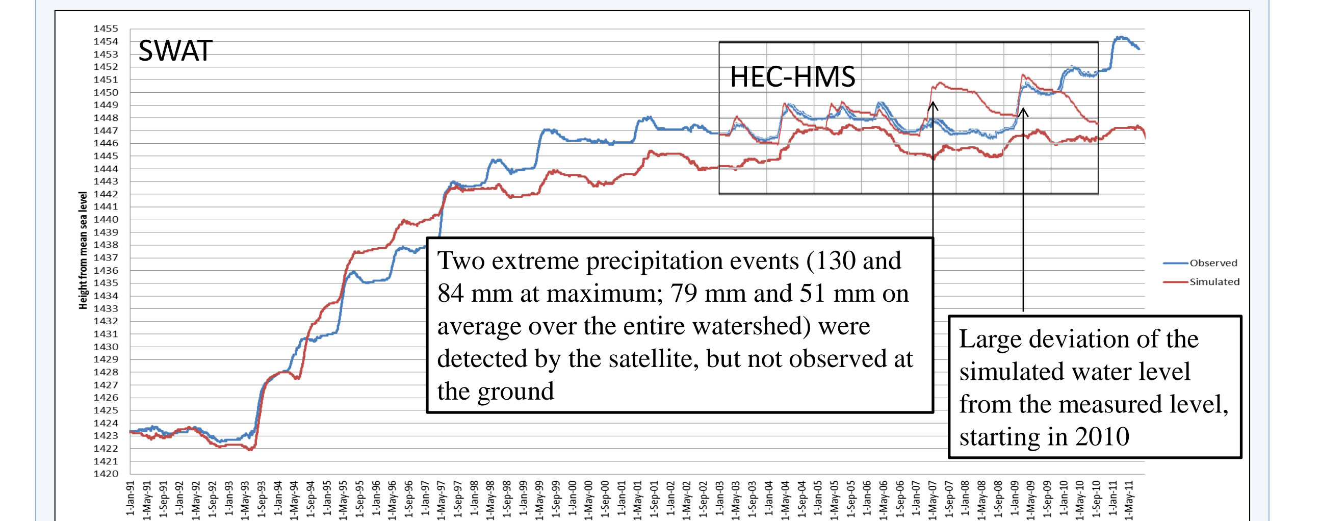
Figure 8. SWAT and HEC-HMS simulations of the Devils Lake water level (ft. amsl). Starting in 2010, both models heavily underestimate the lake water level.
