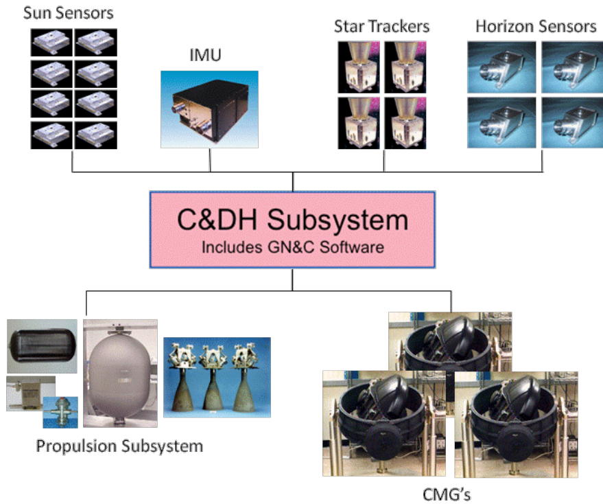
Figure 6.—AD&C block diagram.
