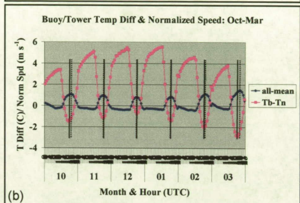
Figure 12. Plot of the hourly differences between the buoy and tower network mean 1.8 m temperatures ( T_b - T_n ), and the hourly mean wind speed normalized by the monthly mean wind speed (all-mean), valid for the months of (a) April to September, and (b) October to March. Solid vertical lines represent the time of minimum T_b - T_n (i.e. time of maximum tower temperatures) and dashed vertical lines represent the time of the maximum mean wind speed.
