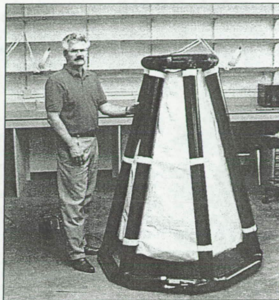
Prototype of the Inflatable Aeroponic System for space and micro-gravity food production
