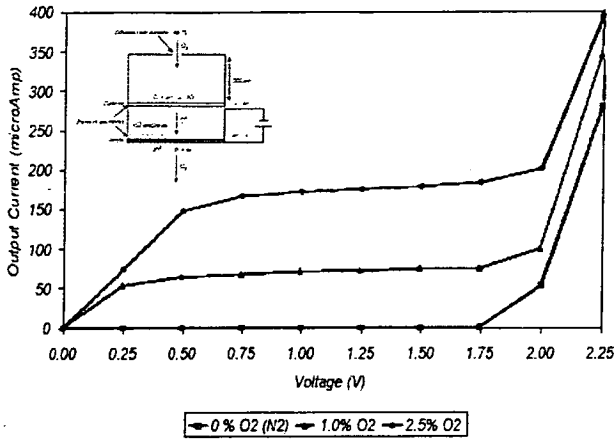
Plot 1. O 2 Limiting Current Profile
