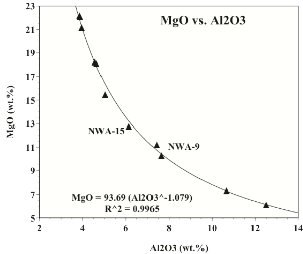
Figure 2. MgO v. \text{Al}_2\text{O}_3 for NWA 6162 experimental glasses. NWA-9 and NWA-15 were both performed at 1300°C. NWA-9 was at temperature (7 days) for twice as long as NWA-15 and consequently lost \sim 0.75 wt.% \text{Na}_2\text{O} . All experiments are excellently fit by a single regression.
