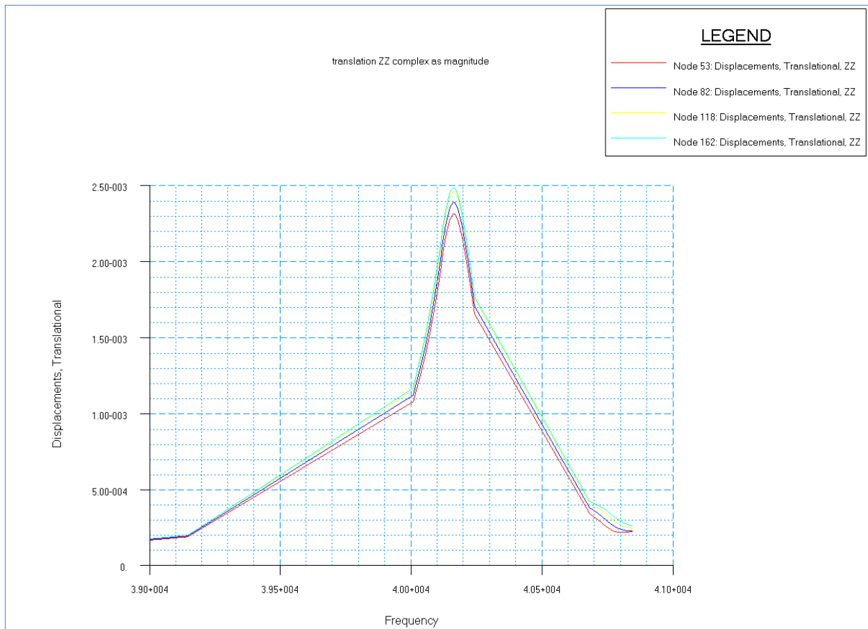
Figure 2. Peak Frequency Response of Highest Responding Nodes in Beam/Plate model
