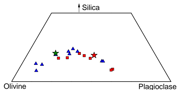
Figure 3 Olivine-silica-plagioclase pseudoternary demonstrates the relationship between the experimental liquid compositions (red squares) and calculated parental melt compositions for shergottite meteorites (Shergotty, Zagami, EETA79001 A&B, ALHA 77005, Los Angeles, LEW 88561, DAG 476, Dhofar 019 [15-20]) (blue triangles). Y98 and QUE [2, 1] are represented by green and red stars respectively.
