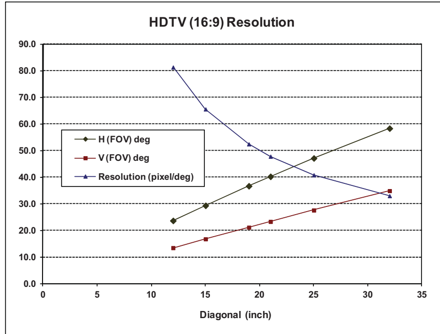
Figure 6: Visual Acuity and FOV vs. Display Size, using HDTV Resolutions
