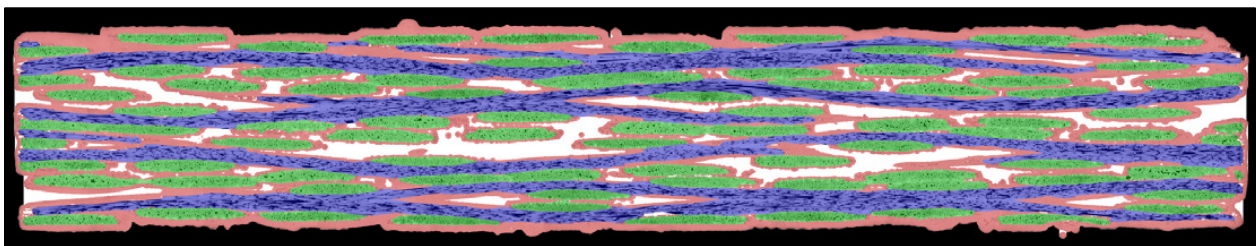
Figure 6.—Composite constituents isolated with an automated procedure utilizing binary morphological operations. Isolated constituents are overlaid on the image of the cross section. Transverse sectioned tows—green; longitudinally sectioned tows—blue; matrix—red; inter-tow porosity—white; and outside specimen—black.
