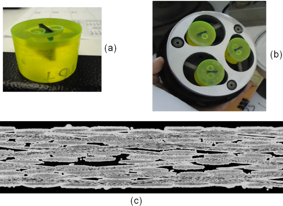
Figure 3.—Specimen mounted in epoxy for polishing (a), three specimens in the polishing apparatus (b), and an example of a polished CVI SiC/SiC composite cross section (c).
