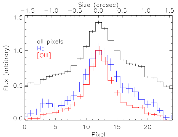
FIG. 5.— Spatial profiles of the \text{H}\beta (blue line) and [\text{OIII}] (red line) emission lines, along with the entire spectrum (black line, offset by +0.4 in flux). Each 1D profile is extracted along the cross-dispersion direction, using the three pixels ( 140\text{\AA} ) about each line center for the emission lines or the entire wavelength range for the entire spectrum profile. The \text{H}\beta profile is more extended than the [\text{OIII}] profile with 98.1% confidence, suggesting that at least some of the objects have a compact AGN contributing to the [\text{OIII}] emission.
