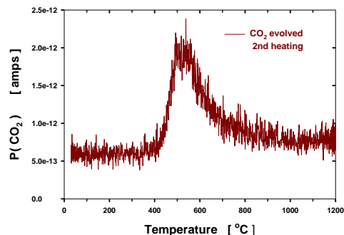
Figure 3. Measured CO 2 release for the second heating of a 125-250µm calcite sample.
