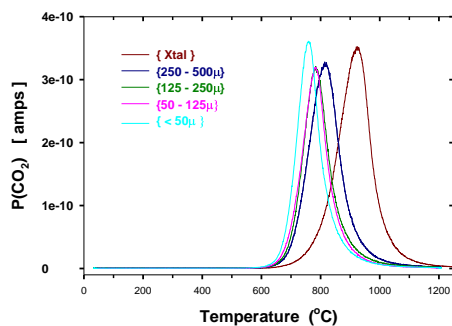
Figure 1: Evolved CO 2 for a 31 mg single crystal of calcite and several particle sizes. These experiments were performed at 30 mb using a He carrier gas at 3 secm.
