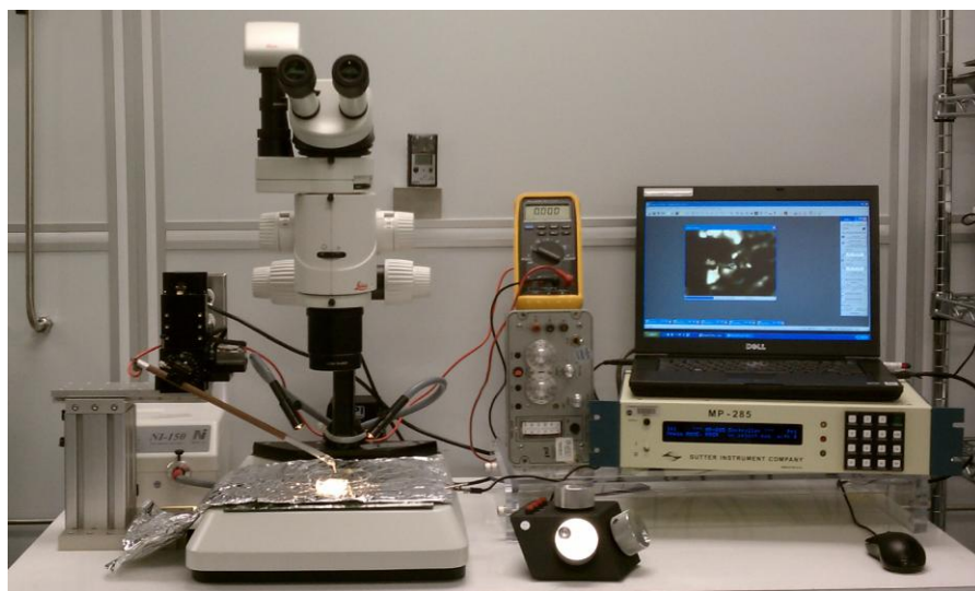
FIGURE 2. Prototype of the voltage-assisted micro-manipulator system to be used to handle and transfer sub-mm asteroid grains. It has been operated successfully to manipulate olivine test grains in this size range.
