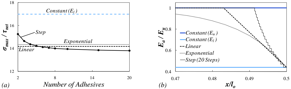
Figure 11.—Increasing the number of adhesives used for a discretely graded adhesive and optimizing the adhesive spacing lowers the maximum adhesive peel stress; (a) stress versus number of adhesives, and (b) modulus at the end of the adhesive for 20 steps compared with the other functions.
