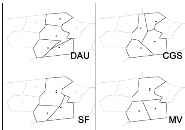
Figure 2: Four Examples of Algorithm-Generated Airspace Designs for a 4-Sector Traffic Scenario (N.B. MV has an airspace configuration that first combined sectors and then split the sectors vertically by altitudes.)
