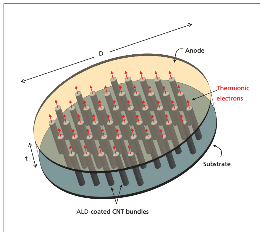
Schematic representation of the Thermionic Power Cell (TPC) with alkali-metal coated CNT bundles to enhance thermionic emission.
