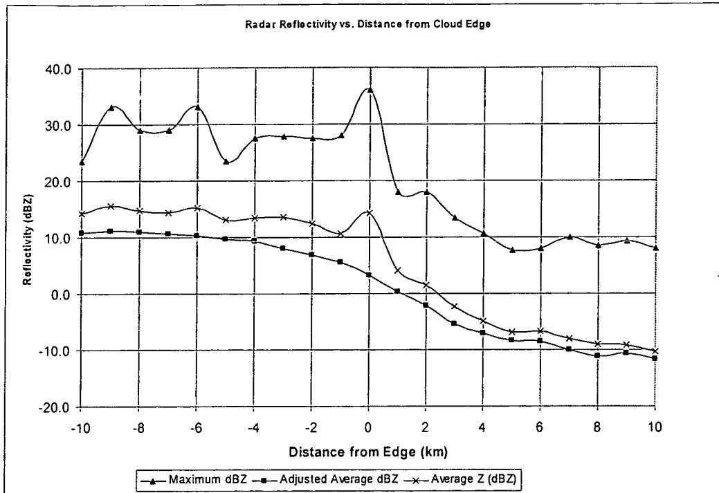
Figure 2. Maximum and average radar reflectivity (dBZ) as a function of distance (km) from the edges of anvil clouds. Positive distances are in clear air, and negative distances in cloud.
