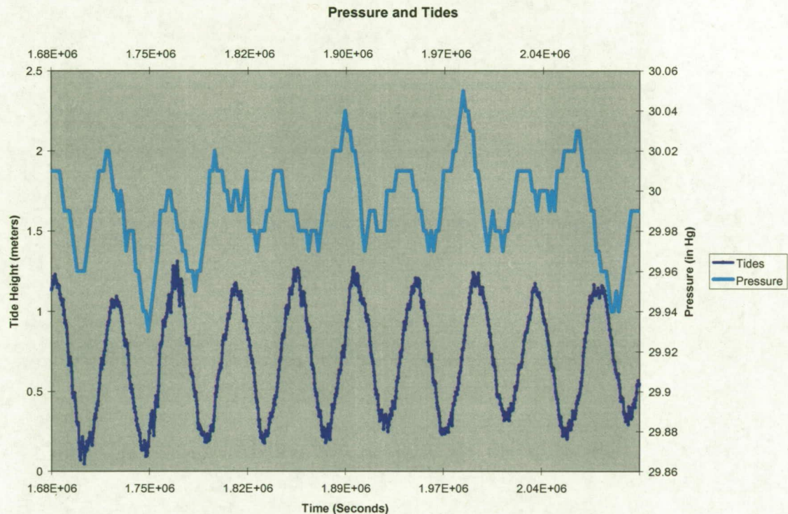
FIGURE 7. The graph shows the tide height and barometric pressure. (X-axis: JCD 236 at 0:00:00 GMT to 241 0:00:00 GMT)
