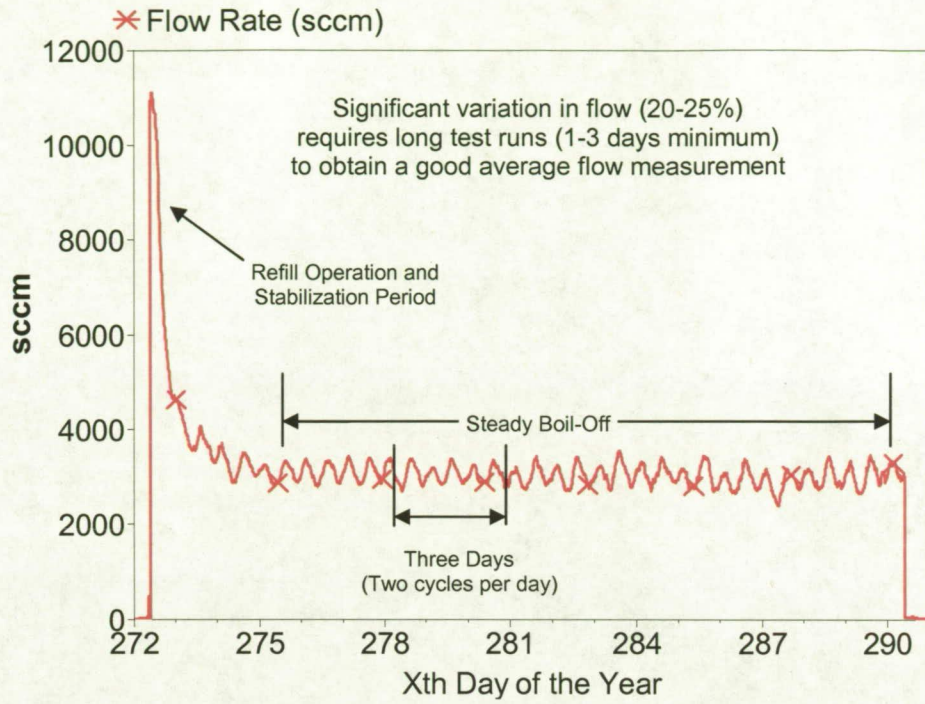
FIGURE 2. Graph showing typical data collected during a boil-off test.
