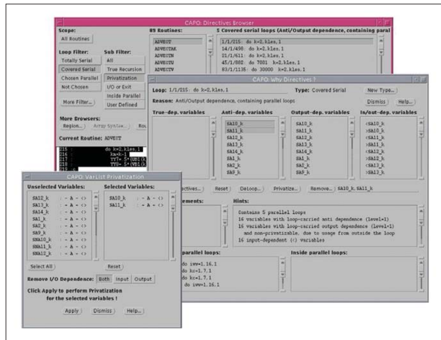
The Main GUI (Directives Browser) for CAPO.
