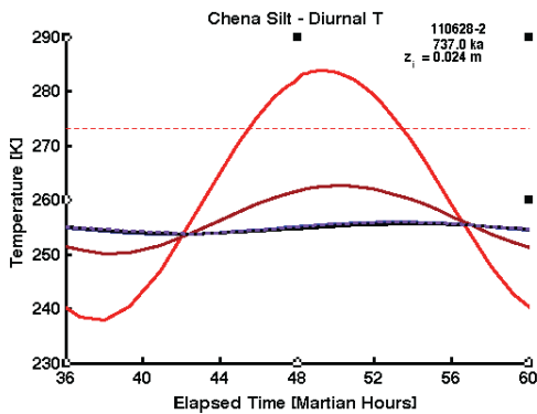
Figure 3. Chena Silt -737 ka bp. Same as Figure 1 .
