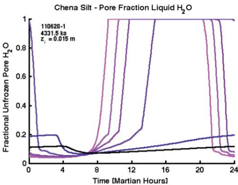
Figure 2. 4.33 Ma bp. Soil: Chena Silt. The fraction of melted H 2 O in soil pores.
