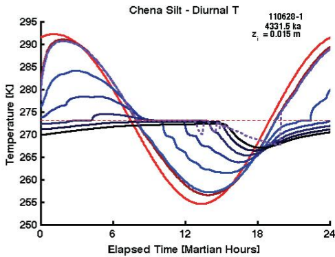
Figure 1. 4.33 Ma bp. Soil: Chena Silt. Temperature of the surface layer and the uppermost 6 nodes in the ice.
