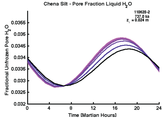
Figure 4. Chena Silt 737 ka bp. Same as Figure 2
