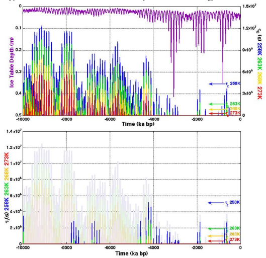
Figure 5. Different ice temperature histories that result from differing assumptions about the polar cap.
