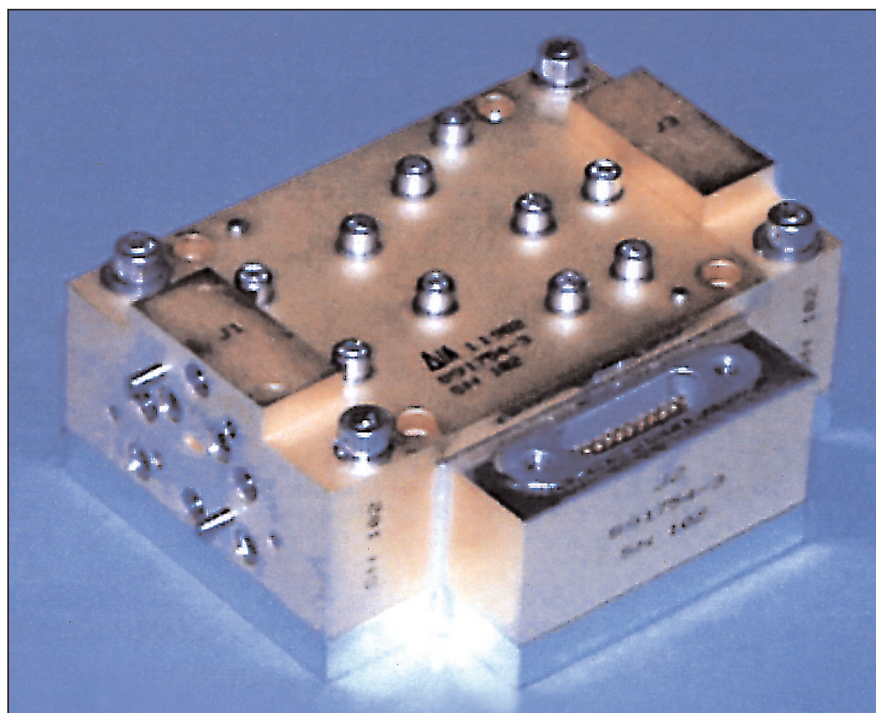
This Photograph Shows One of the Amplifiers described in the text. A WR-10 waveguide input port is on the left end. The output port is on the right end, facing away. DC input and sensing conductors enter the package via a 21-pin connector. (Module dimensions: 20 × 49 × 60 mm.)
