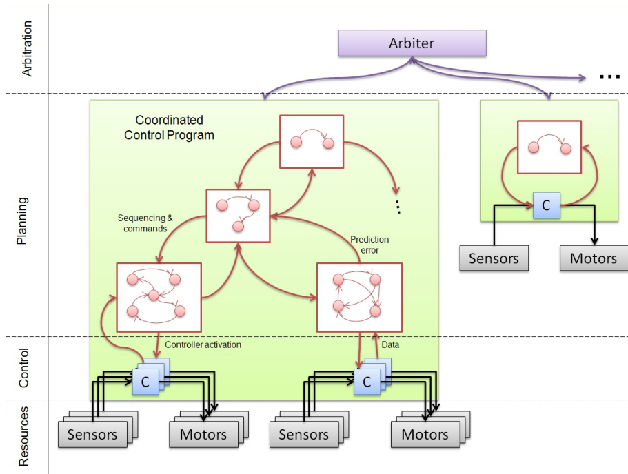
Figure 2: R2's state of the art multi-tiered control architecture.
