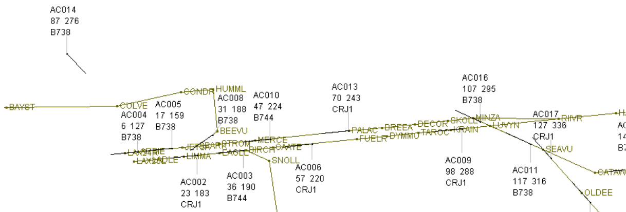
Figure 6. Simulation of scenario with trajectory changes triggered to create an off-nominal situation.
