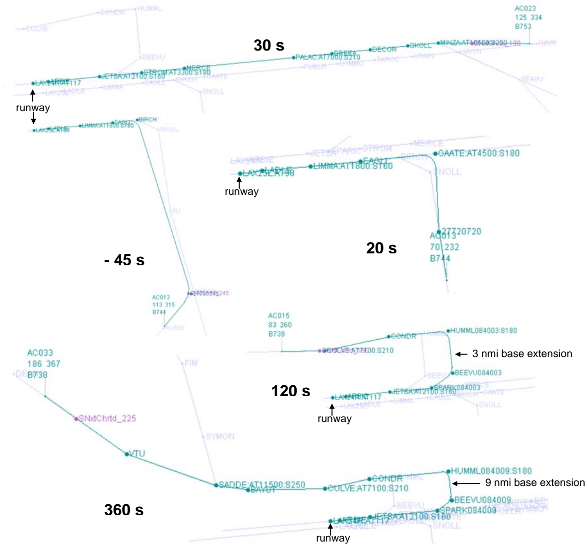
Figure 13. Trajectories generated by TRAC to yield the indicated advance or delay.
