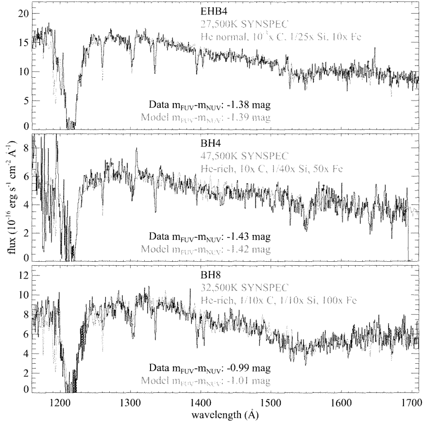
Figure 4. Representative spectra from our sample: a normal EHB star ( top panel ), a BH star ( middle panel ), and one of the unusually red subluminal stars ( bottom panel ). In each panel, we also show a synthetic spectrum (grey curve) that matches both the observed spectrum (Brown et al. 2011) and UV photometry (Brown et al. 2001). Compared to the normal EHB stars, the BH stars are hotter and have stronger helium and carbon lines, as expected if the BH stars formed via flash mixing. The BH stars all exhibit enhanced iron-peak abundances, while the normal EHB stars are mixed, with some enhanced and others not. Some subluminal EHB stars are much redder than expected (see Figure 3), but their red colors can be explained by a large enhancement of iron-peak elements, presumably from radiative levitation.
