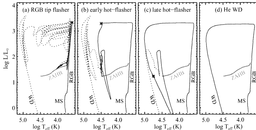
Figure 1. Various evolutionary paths for producing an HB star (from Brown et al. 2010). The zero-age HB (ZAHB) phase is highlighted in grey, while the pre-ZAHB evolution (solid curves) and post-ZAHB evolution (dashed curves) are in black. The peak of the helium-core flash is marked by an asterisk. The four panels show the evolution for progressively larger amounts of mass loss on the RGB. The evolution in the first two panels produces canonical HB stars in which the H-rich surface composition does not change during the helium-core flash. In the third panel, the helium-core flash occurs on the WD cooling curve, producing a flash-mixed star having a surface composition highly enriched in helium and carbon and a temperature significantly hotter than the canonical HB. In the fourth panel, the helium flash never occurs and the star dies as a helium WD.
