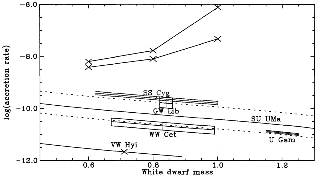
Fig. 3.— The inferred accretion rate at the highest flux of the optically thin X-ray emission, plotted against the white dwarf mass (see text for object-by-object details). Also shown are the theoretical curves of optically thin-to-thick transition from Popham & Narayan (1995).
