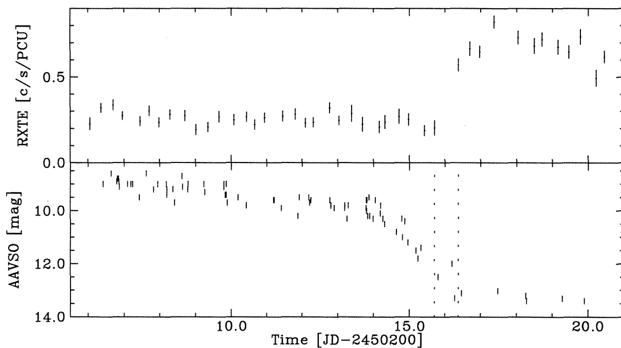
Fig. 1.— The X-ray (top panel) and visual (bottom) light curves of VW Hya during 1996 May. The X-ray data were obtained with RXTE PCA while the optical data were collected by amateur observers and compiled by AAVSO. Two vertical dashed lines mark the time of the last “outburst” and the first “quiescent” X-ray points (see text).
