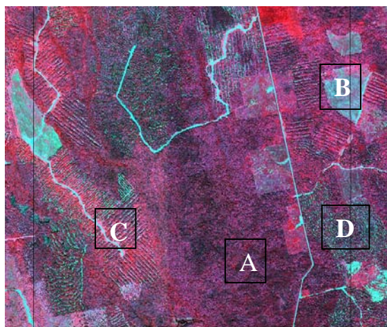
Fig. 1. IKONOS image showing undisturbed forests (A) and those with the clear cut (B), strip cut (C) and selective cut (D).
