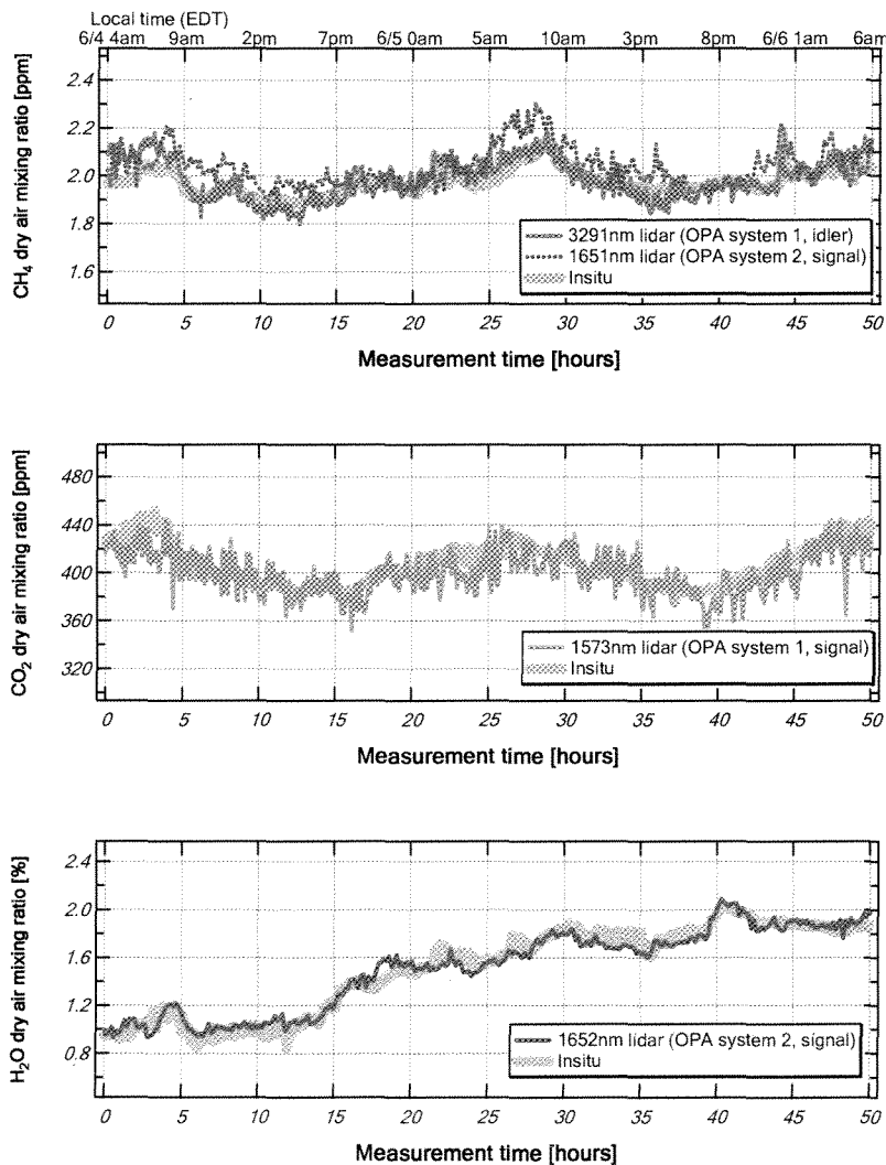
Figure 6. Simultaneous measurements of the diurnal variations of atmospheric CH 4 (top), CO 2 (middle), and H 2 O (bottom) measured with the two OPA lidar systems and an in-situ sensor.
