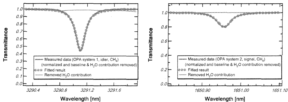
Figure 5. Examples of measured scan data and fitting results. \text{CH}_4 measurement at 3291.1 nm (left) and 1650.9 nm (right) are shown. The scan data was averaged, divided by the signal from the integrating sphere, and further
