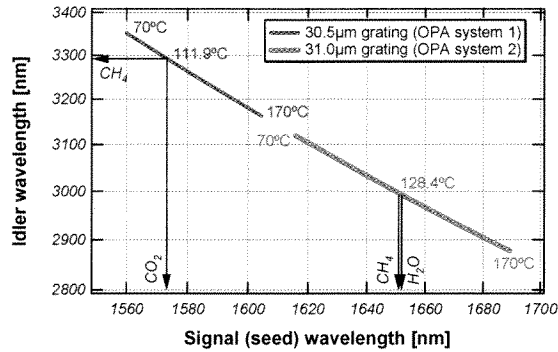
Figure 3. Tuning curves of the two MgO:PPLN crystals used in the two OPA systems.
