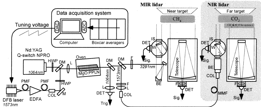
Figure 1. Experimental diagram. A MgO:PPLN crystal is pumped and seeded by a Q-switch Nd:YAG NPRO and a DFB laser, respectively. In OPA system 1 (1573 nm seed), both signal and idler are used for lidar measurement as shown in this figure. In OPA system 2 (1651 nm seed), only signal is used for lidar measurement and there is no EDFA and MIR lidar. EDFA: Erbium-doped fiber amplifier, HWP: half wave-plate, M: mirror, DM: dichroic mirror, L: lens, F: wavelength-selecting filter, COL: fiber collimator, IS: integrating sphere, W: wedge, DET: detector, BE: beam expander, PMF: single-mode polarization maintaining fiber, MMF: multi-mode fiber, ADC: analog-to-digital converter, DAC: digital-to-analog converter, Trig.: trigger signal for boxcar averagers, Sig.: Signal input for boxcar averager.
