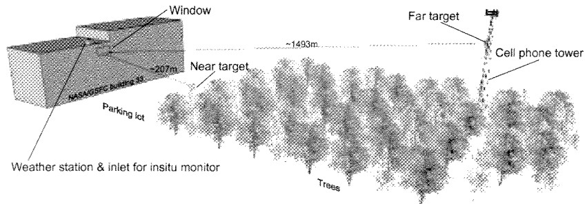
Figure 2. Schematic view of two open paths. Only the MIR lidar (OPA system 1, idler) used the near target. Other NIR lidars (signals of OPA system 1 and 2) used the far target.
