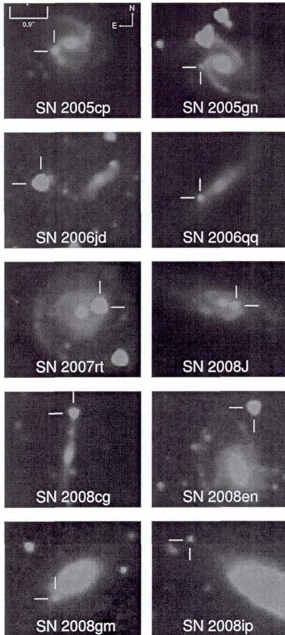
Figure 1. False-color 3.6 \mu\text{m} and 4.5 \mu\text{m} combined Spitzer /IRAC images of the 10 SNe II n discovered by our survey (P60122) to exhibit late-time mid-IR emission.
