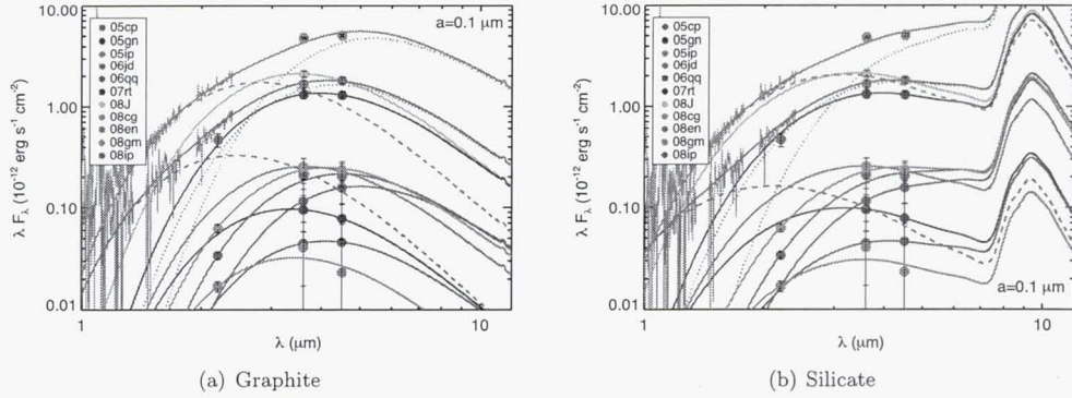
Figure 5. Best fits of Equation 1 (both graphite and silicate compositions) to the combined near-IR and mid-IR data. A warm ( \sim 400\text{--}800\text{ K} ) dust component fits most observations well. SNe 2006jd and 2005ip (those with near-IR spectra) are better fit by a multi-component model, where a second, hotter component dominates the near-IR flux. The most obvious feature differentiating between the graphite and silicate models is the 9\ \mu\text{m} silicate emission feature. The warm IRAC data do not extend beyond \sim 5\ \mu\text{m} , limiting any distinction between the two compositions.
