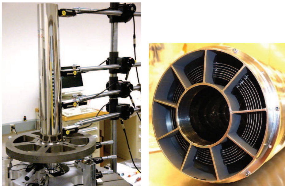
Figure 4. Left: Photograph of the mirror shell assembly integration stand. The stand makes use of Keyence proximity sensors, accurate to 0.1 micron, to monitor the circularity of the shell in real time throughout the bonding process. During assembly the shells are lowered in place from smallest to largest and held at three points by micropositioners which are adjusted to maintain circularity. A UV-cure epoxy is used to fasten the shell clips to the spider spokes, above which the shell is suspended. Right: A photograph of a completed FOXSI telescope module.
