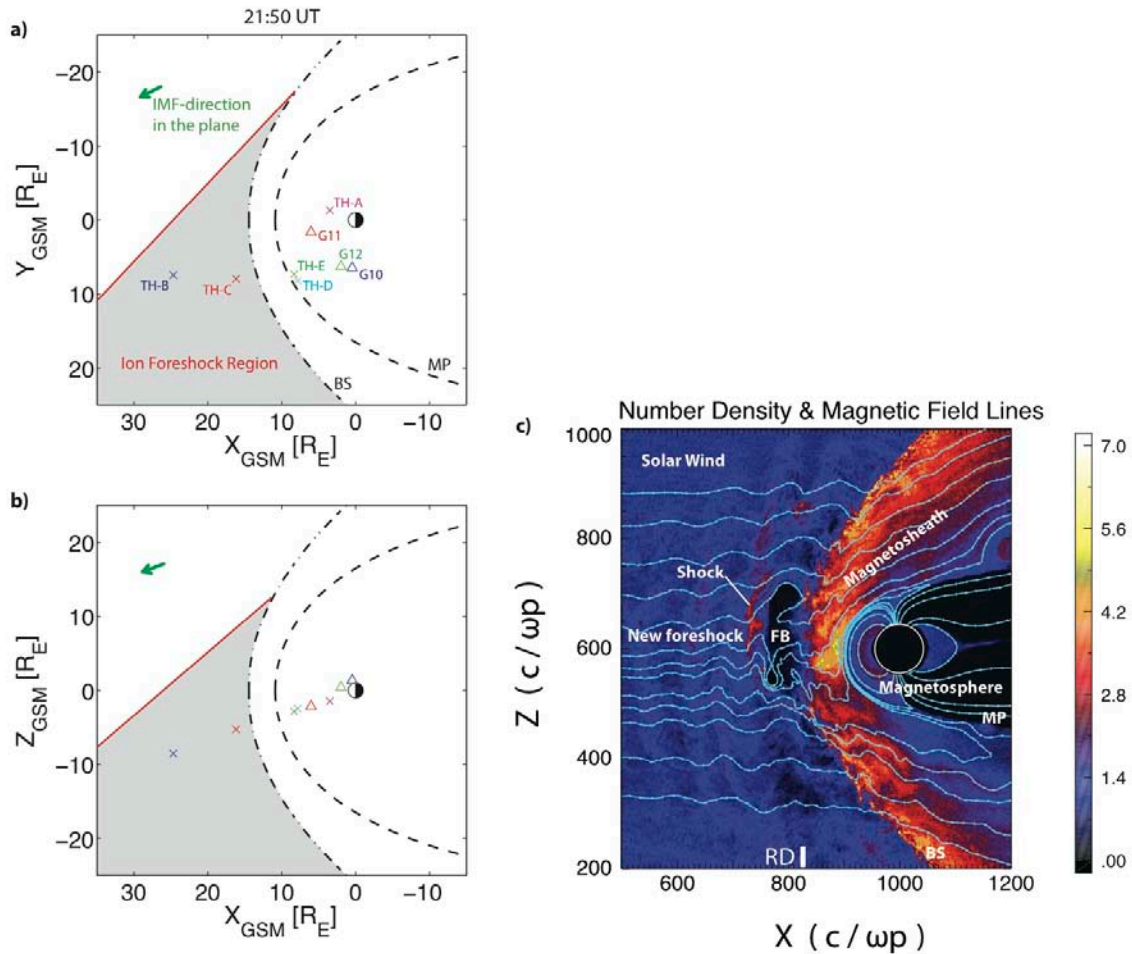
Figure 1: a) and b) THEMIS and GOES locations at 21:50 UT on 14 July 2008. Magnetopause (MP) and bow shock (BS) models ([Shue et al., 1997], [Fairfield, 1971]) are shown with the dashed lines. Note that North America spans from pre-noon to post-dusk (+X, +Y quadrant) at this time. The shaded gray region shows the estimated ion foreshock region, and the green arrows show the IMF direction in each plane. c) 2.5-dimensional hybrid simulation results of a foreshock bubble ([Omidi et al., 2010]) showing number density in color, normalized to the solar wind, and magnetic field lines. The X and Z axes are in units of the ion skin depth, where c is the speed of light and \omega_p is the ion plasma frequency. The axes are in simulation coordinates where the origin is located at the lower left corner of the simulation box. The white circle around the Earth represents the simulation's inner boundary, which is a dipole inside a perfectly conducting sphere. The foreshock region here is originally upstream of the subsolar point, since the IMF in the simulation is primarily in the X-direction. Note the wave activity in this region, which is a typical feature of the ion foreshock and is evident in both the density and the magnetic field lines. A rotational discontinuity (RD) in the IMF is indicated on the figure and results in the formation of a foreshock bubble (FB), which is the large density depletion region around the subsolar point. The shock wave associated with the FB is apparent in the enhanced density band at the upstream edge of the bubble. Note also that the field directions within the bubble can become highly distorted.
