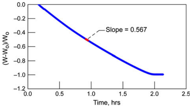
Fig. 5 Typical weight loss curve for rayon-derived carbon fiber cloth at 900 °C in air. Note the specimen is consumed at ~2 h
