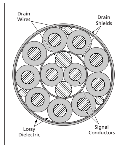
This Cross Section illustrates one of many possible charge-dissipating designs for a cable containing 11 signal conductors.
