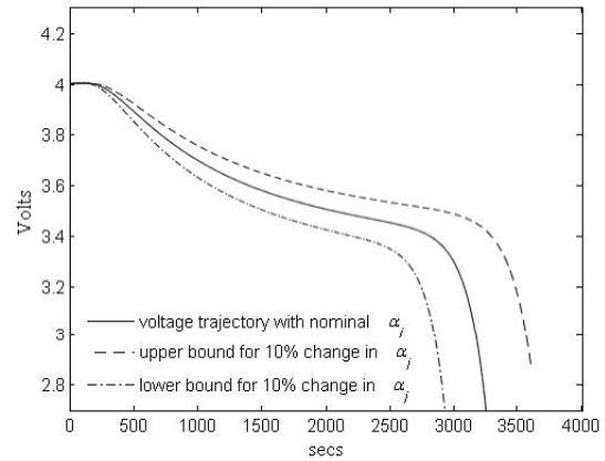
Figure 7. Li-ion discharge trajectories with changes in model parameter estimates.
