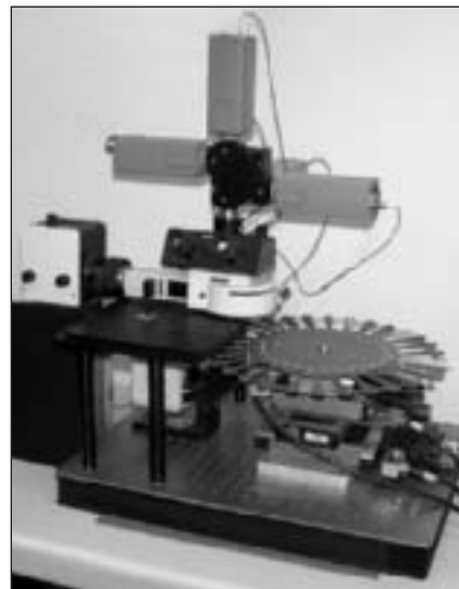
The Original Version of the Automated Fluorescence Microscope included four CCD cameras and dichroic beam splitters for acquiring images in four fluorescence wavelength bands. The instrument was then modified to incorporate a single, more sensitive video camera and a filter wheel for taking a sequential exposures of each microscope field in the fluorescence wavelength bands of interest.
