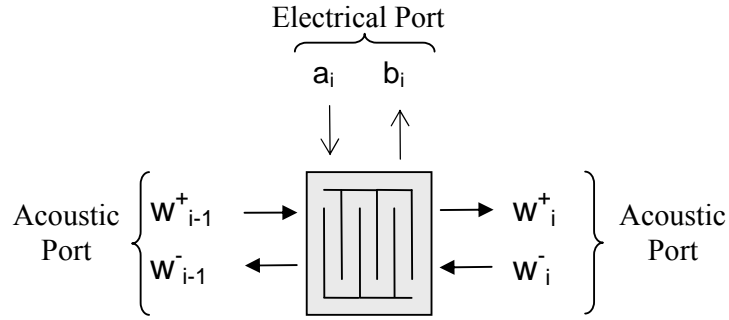
Fig. 3. Transmission matrix model of an IDT.
